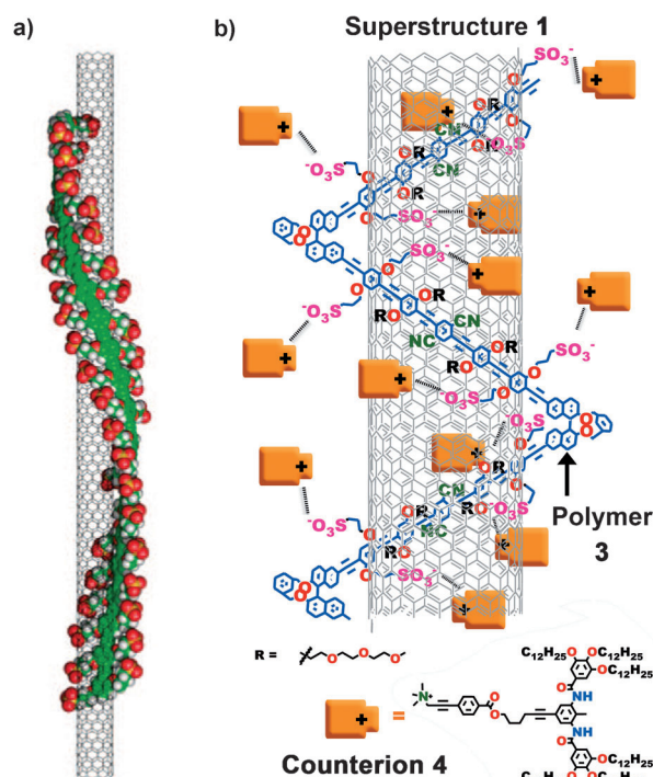
Scheme 1. a) Representation of the [arylene]ethynylene polymer-wrapped SWNT. b) Representation of the ionic self-assembled nanostructure 1 showing the molecular formulas of the anionic conjugated polymer 3 and the amphiphilic cation 4.
